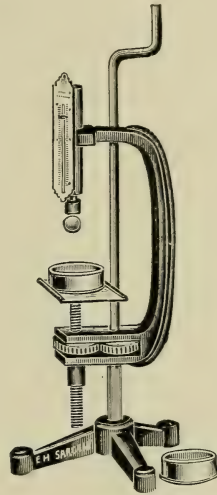
FIG. 172.—Kirschbraun Adhesive Tester.
